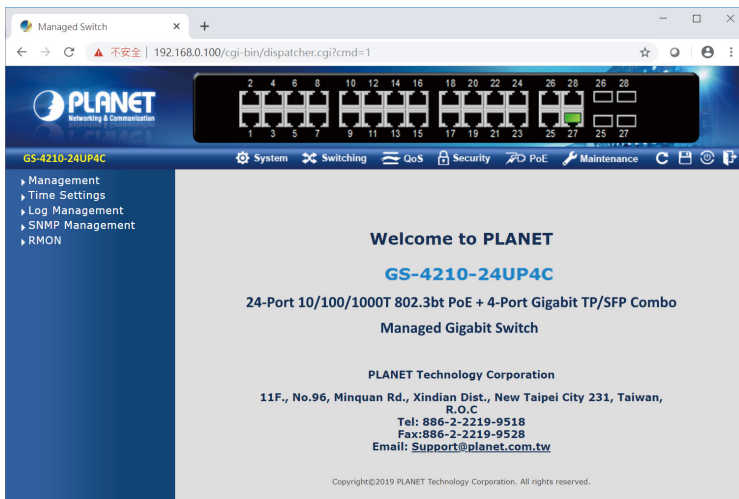
Figure 4-3: Web Main Screen of Managed Switch
